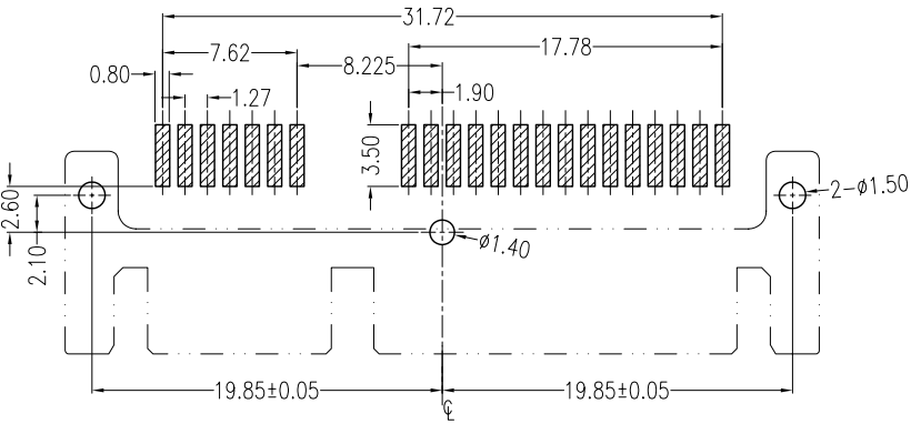
PCB Layout (T=1.60±0.05mm) Top View
